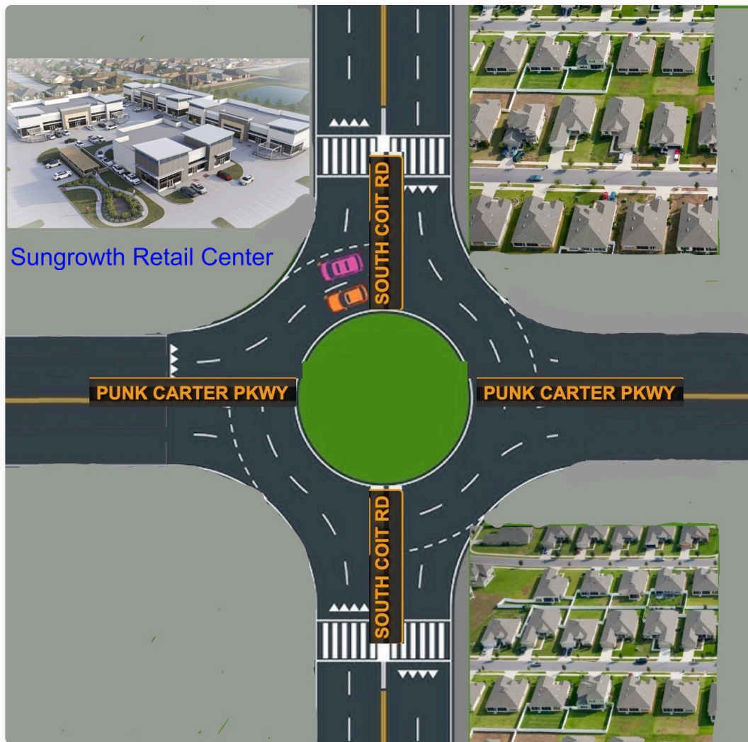
4-Lane Coit Rd & 2-Lane Punk Carter Pkwy Intersection
